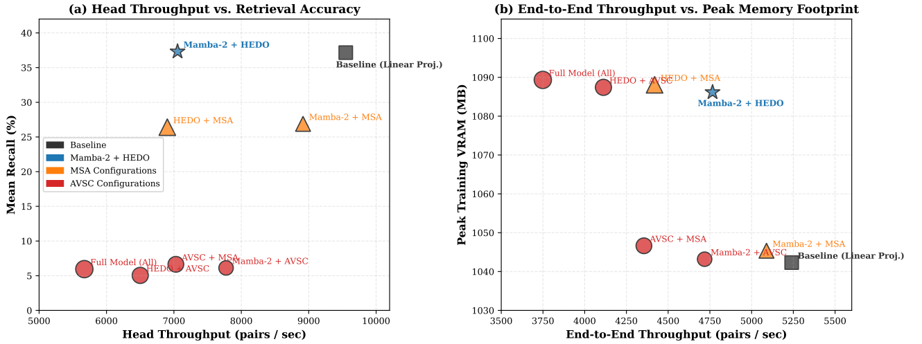
Fig. 4. Efficiency vs. accuracy tradeoffs across all 8 configurations. (a) Head throughput (pairs/s) vs. Mean Recall (%). (b) End-to-end throughput (pairs/s) vs. Peak Training VRAM (MB). Bubble area is proportional to the trainable parameter count (465k to 764k). Mamba-2 + HEDO lies on the observed accuracy-throughput Pareto frontier among the eight evaluated configurations, retaining baseline-level retrieval accuracy at high throughput and low memory.
